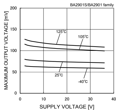
Fig. 67 Maximum Output Voltage - Supply Voltage (IOL=4[mA])
