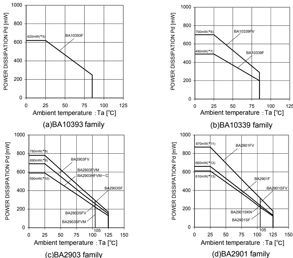
Fig.91 Thermal resistance and derating curve
